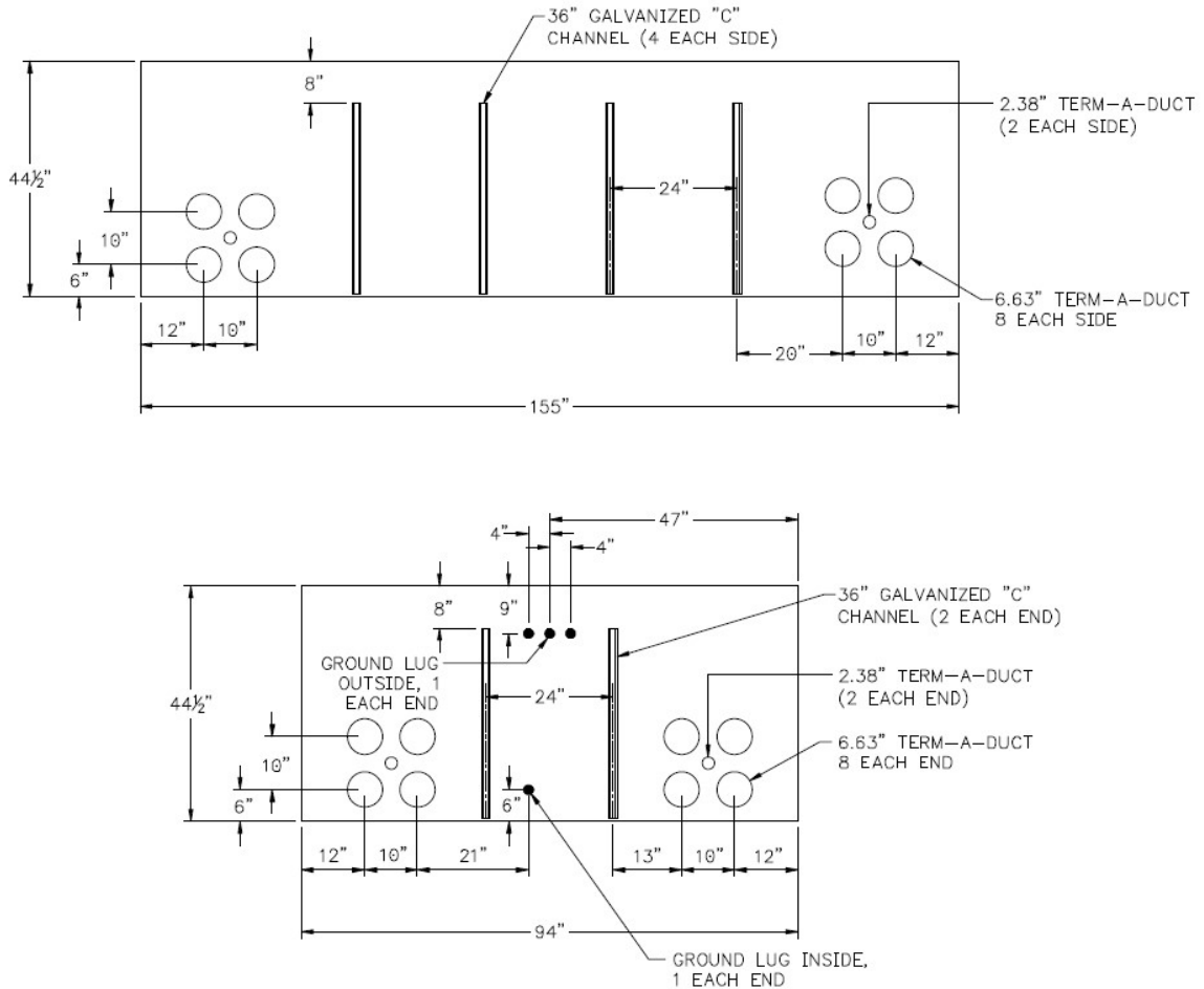
Figure 2—Sleeve TERM-A-DUCT and “C”-Channel Requirement Detail
