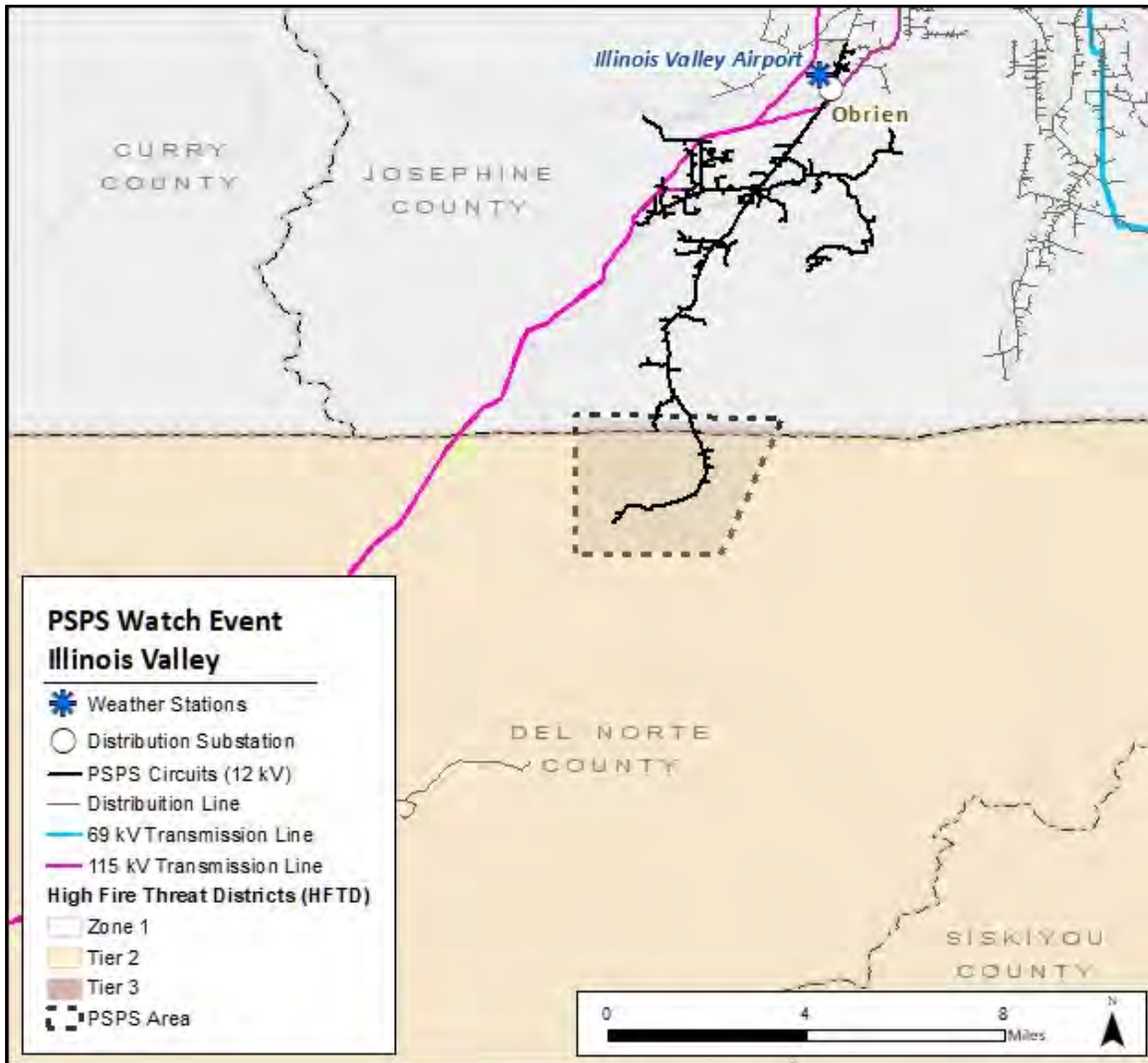
Figure 2. Illinois Valley PSPS watch event area and circuits, HFTD, and weather station locations.
